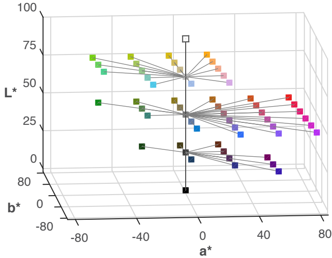
Figure S.2. UW-58 colors plotted in CIELAB color space (figure from [28]). See Table S.5 for the CIELAB coordinates.
